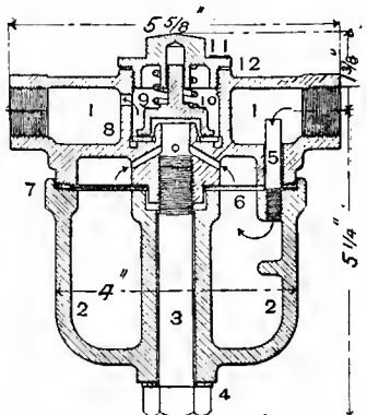
Figs. 3112-3113. Plan and Section. DUST-GUARD AND CHECK-VALVE. (254)
